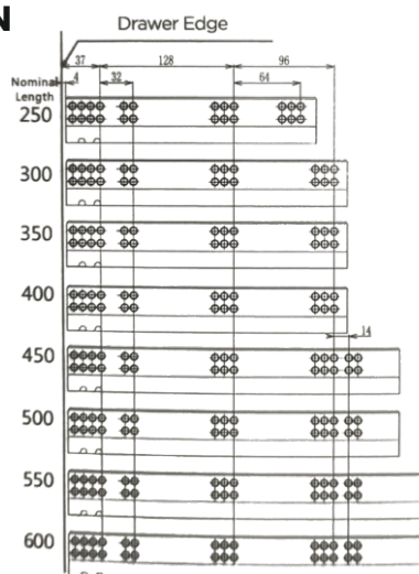
Installation for inner drawer
