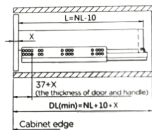
Installation for inner drawer
