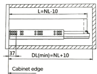
Installation for standard drawer
